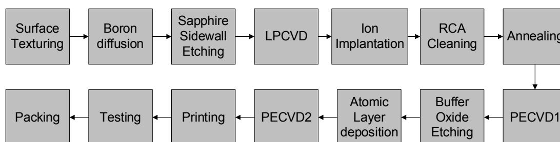
Figure 2 Manufacturing process flowchart of solar cells
